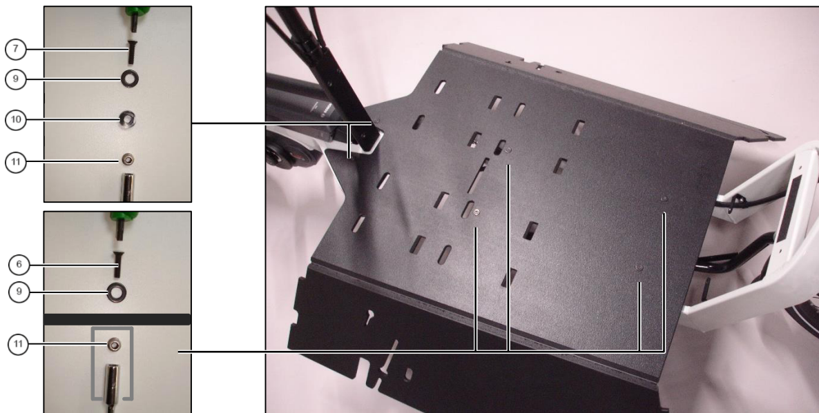
fig. 1: mounting the bottom plate
